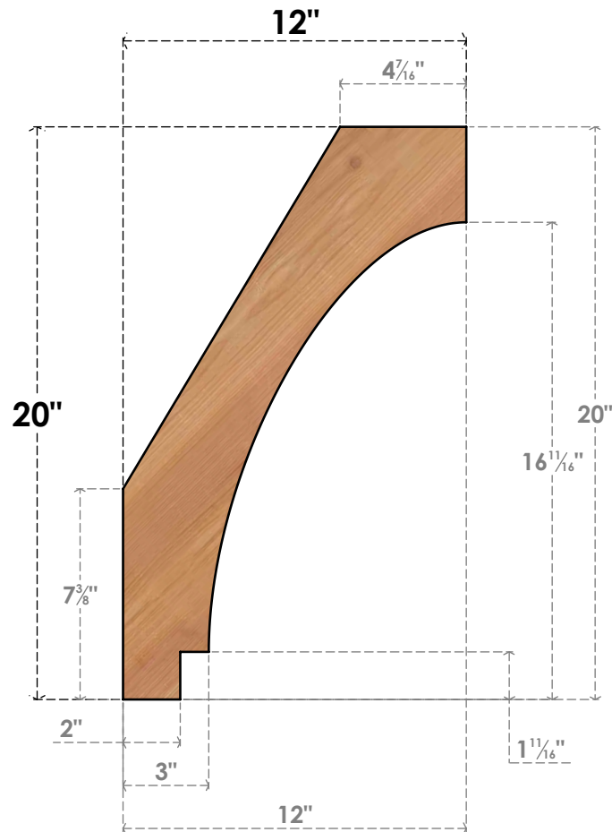
SIDE
